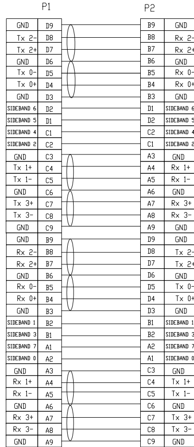
WIRING DIAGRAM
